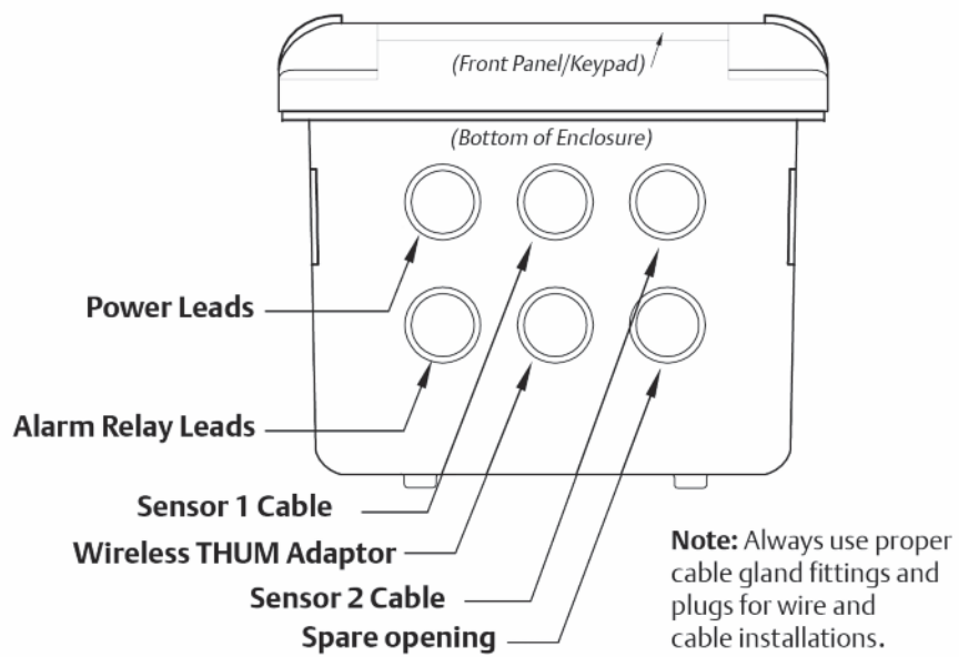
Figure 3-5 56 Recommended Wire Entry and THUM Adaptor Installation
