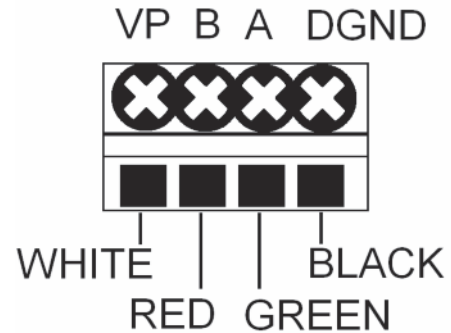
FIGURE 12-4. 4-Lead Terminal Block
