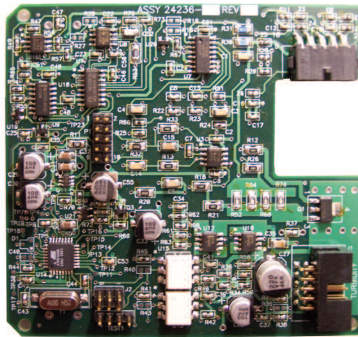
Figure 3-10 Turbidity Signal Board with Plug-in Sensor Connection
