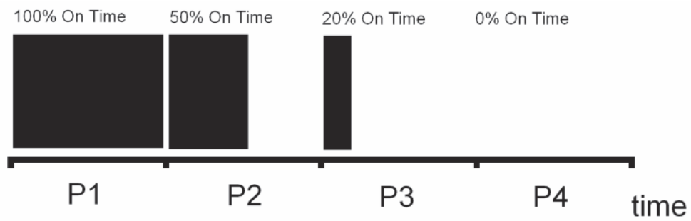
Fig. 8-1 TPC Periods and On Time
