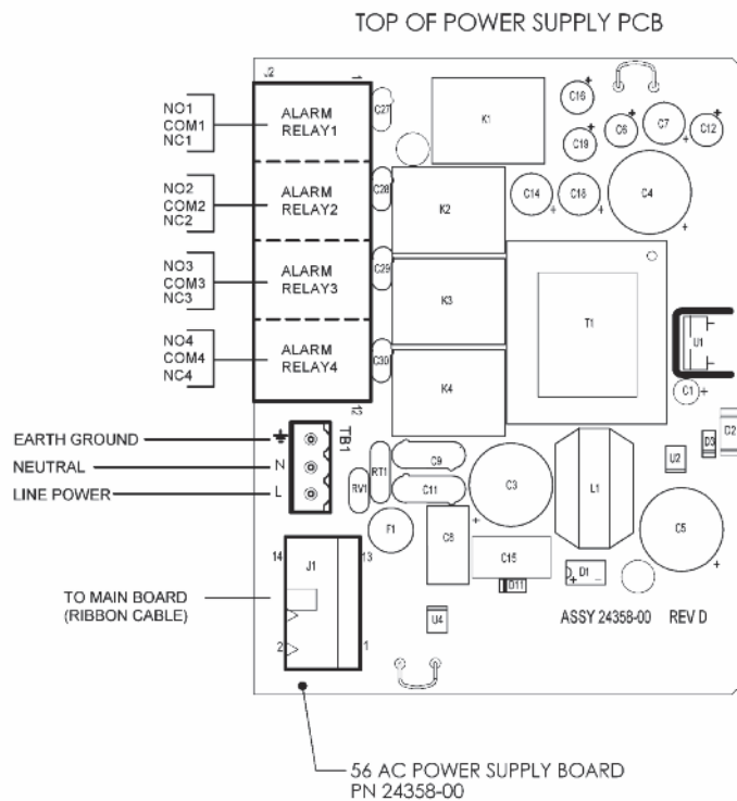
FIGURE 3-2 Power Wiring for 56 85-264 VAC Power Supply (-03 order code) PN 24358-00
