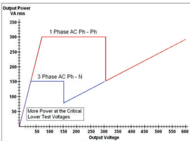
Figure 5: Voltage output power curve
