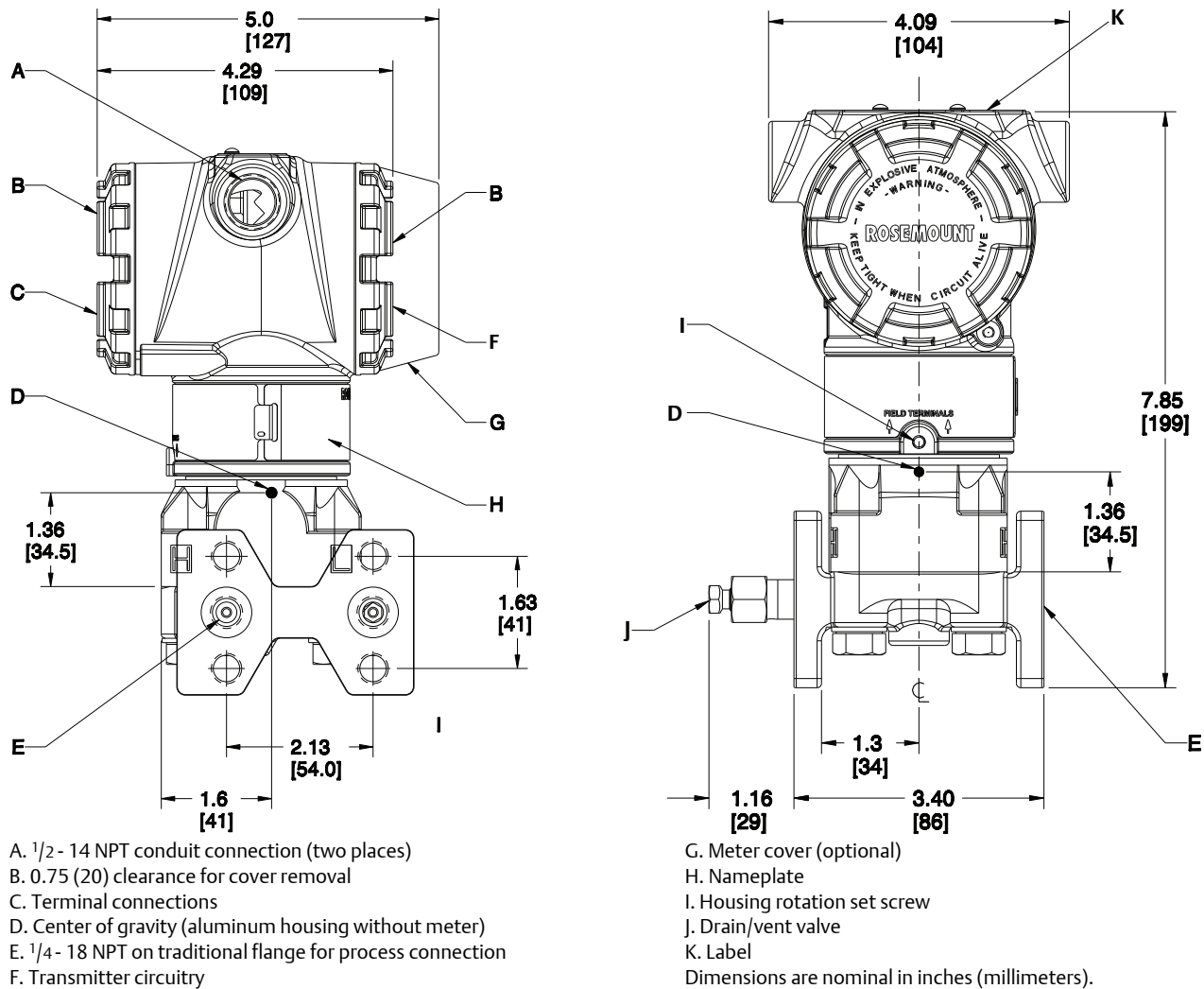
Figure 9. Traditional Flange (Option Code H2) Dimensional Drawing
