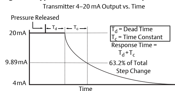
Figure 4. Typical Smart Transmitter Response Time
