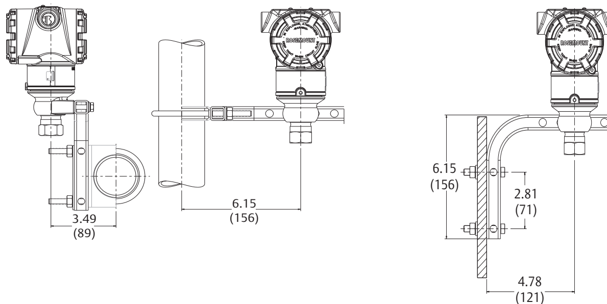
Pipe mounting
